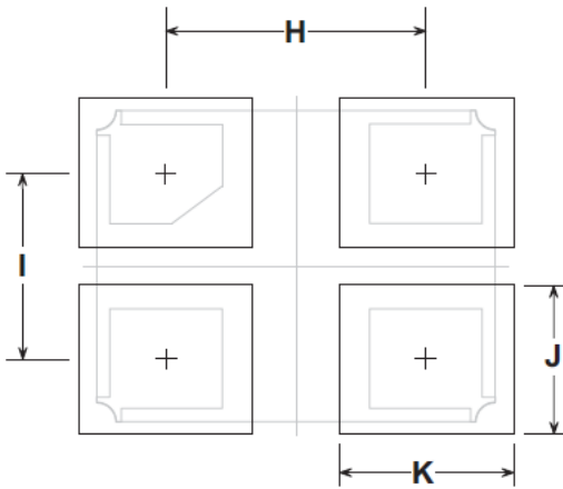
Typical PCB Land Footprint (Top View)
