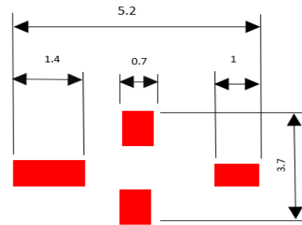
PCB Footprint
