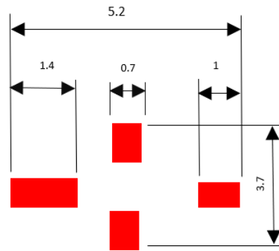
PCB Footprint
