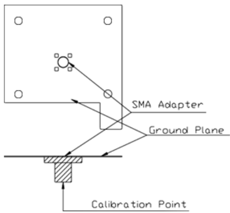
Test Fixture
